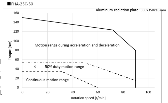
Operable range of FHA-25C-50
