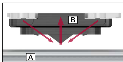
Sensor principle
