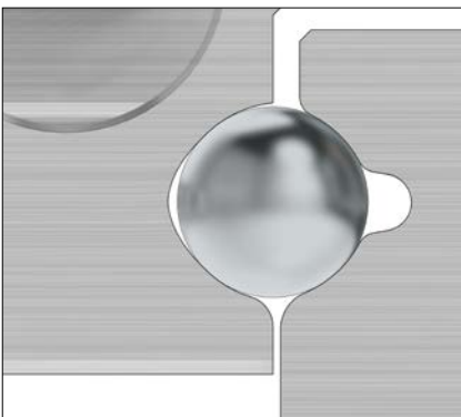
Gothic arc profile of the guideway tracks
