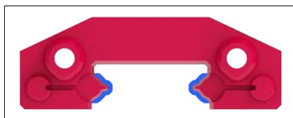
Smooth-running wiper (AL) (blue contour = contact surface)
