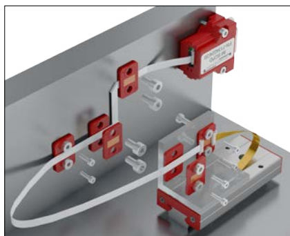
Installation example with FFC extension
