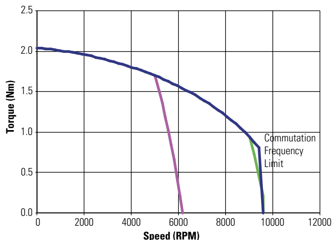
KBM(S)-17X01 ContinuousTorque
