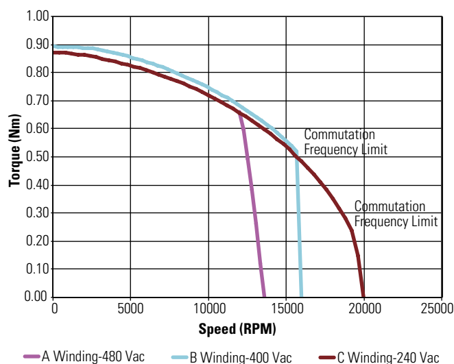
KBM(S)-10X02 ContinuousTorque
