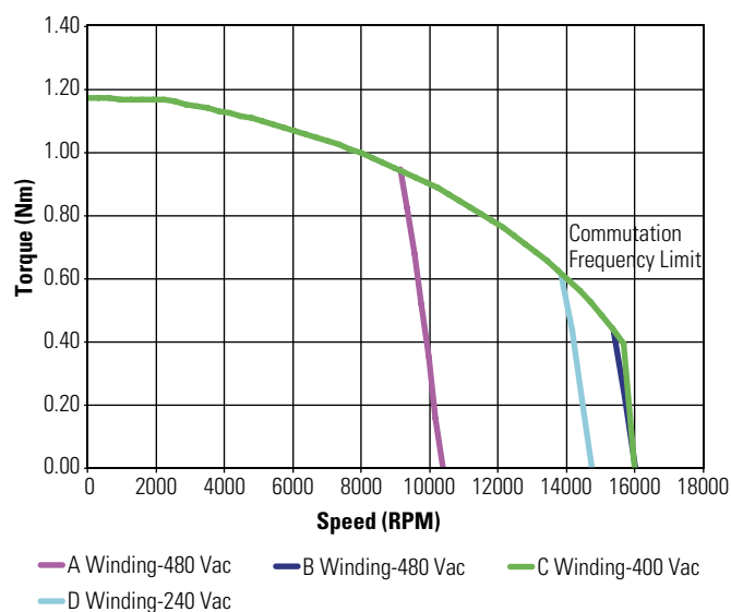
KBM(S)-10X03 ContinuousTorque
