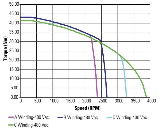
KBM(S)-45X02 ContinuousTorque
