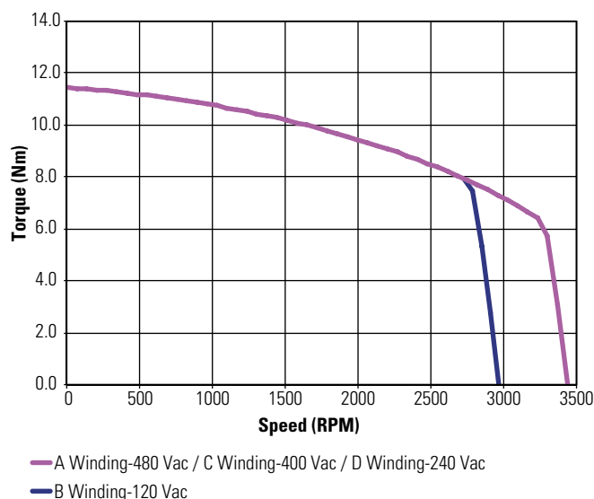
KBM(S)-43X02 Continuous Torque
