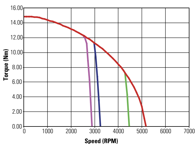
KBM(S)-25X04 ContinuousTorque
