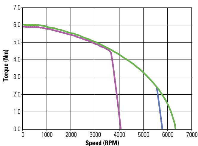
KBM(S)-17X04 ContinuousTorque
