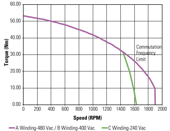
KBM(S)-60X01 ContinuousTorque
