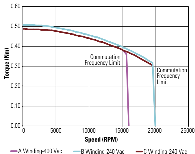
KBM(S)-10X01 ContinuousTorque
