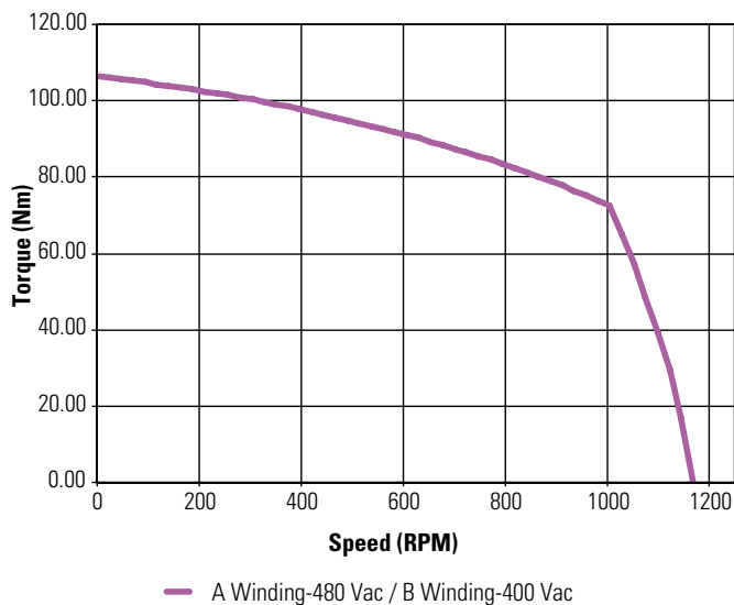
KBM(S)-60X02 ContinuousTorque
