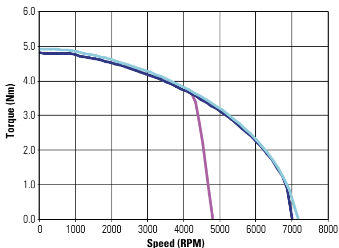
KBM(S)-17X03 ContinuousTorque
