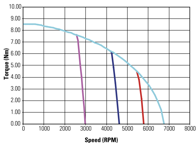
KBM(S)-25X02 ContinuousTorque
