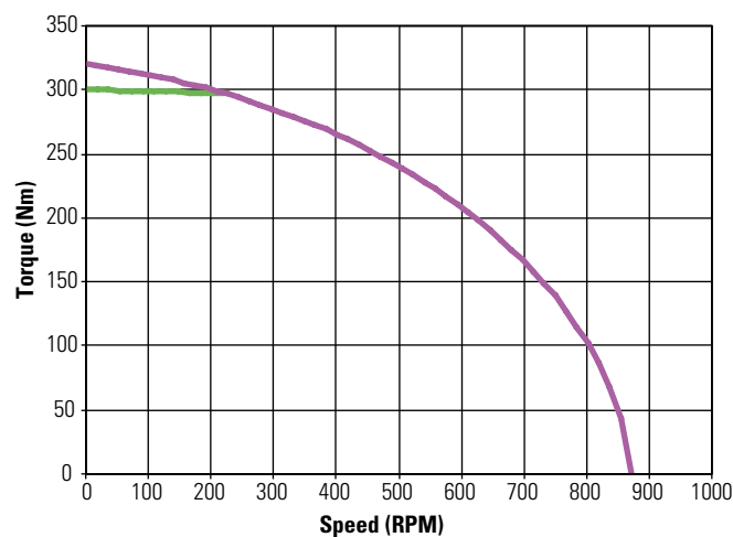
KBM(S)-118X01 ContinuousTorque
