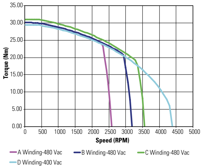
KBM(S)-45X01 ContinuousTorque
