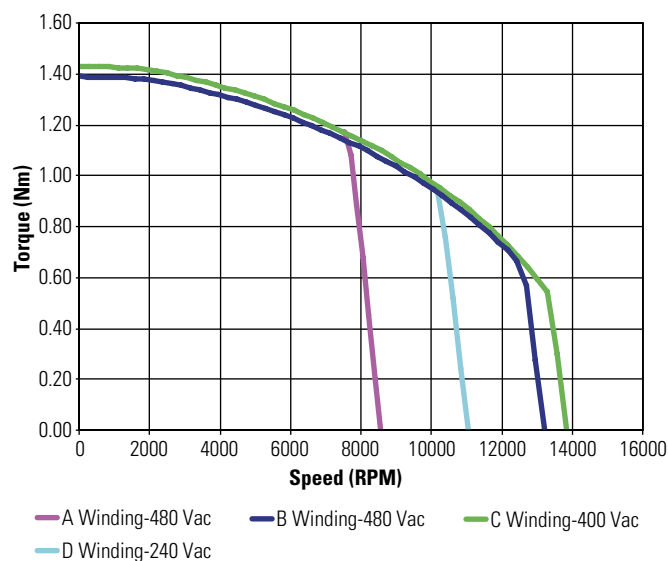
KBM(S)-10X04 ContinuousTorque
