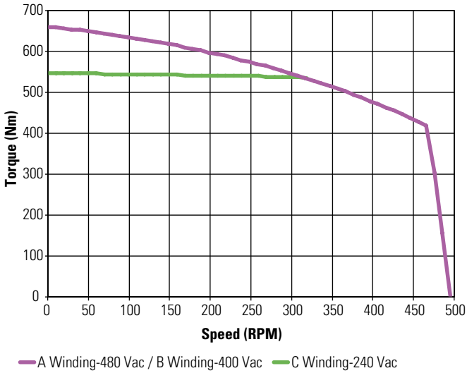
KBM(S)-118X04 ContinuousTorque
