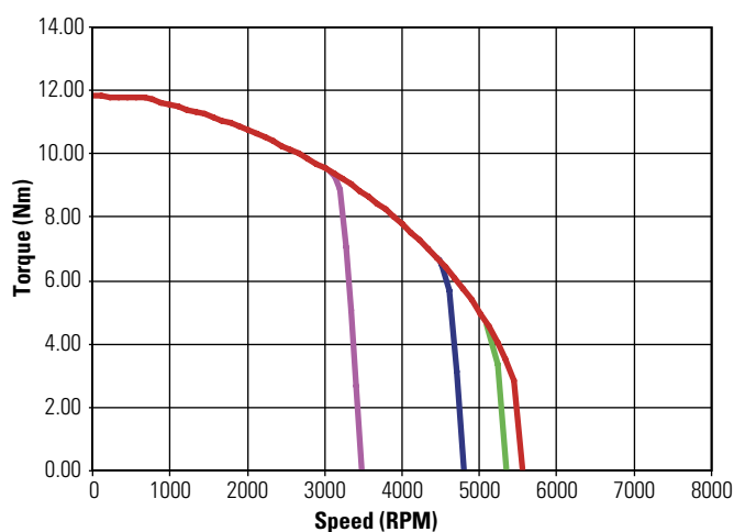
KBM(S)-25X03 ContinuousTorque
