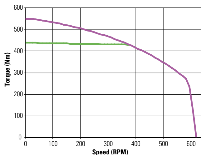
KBM(S)-118X03 ContinuousTorque
