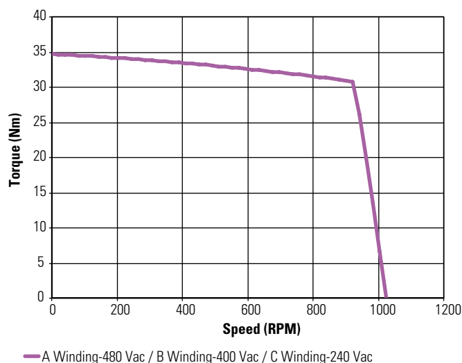
KBM(S)-43X04 Continuous Torque
